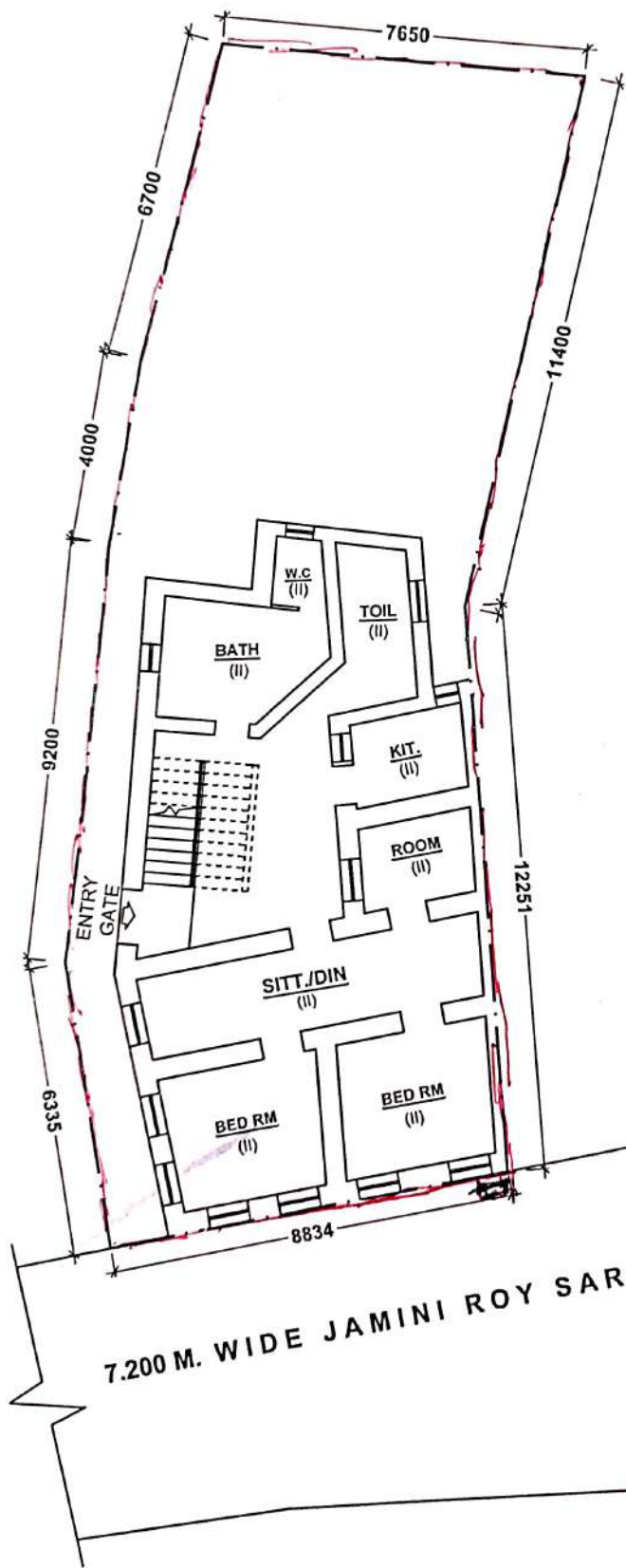
GROUND, FIRST FLOOR EXISTING STRUCTURE PLAN.
